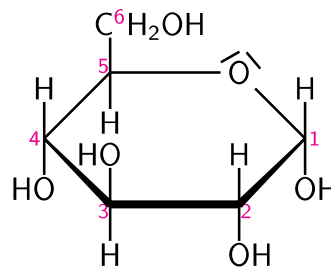
\alpha -D-Glucose
