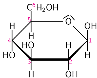
\beta -D-Glucose
